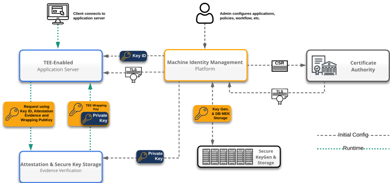
Figure 3 - High-Level Prototype Architecture
