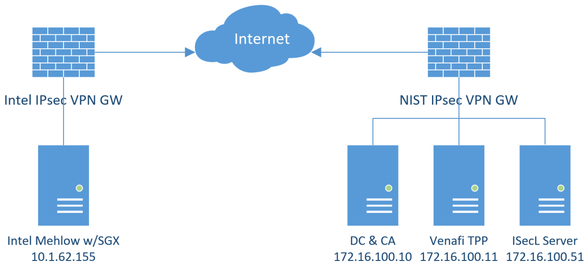
Figure 4 - Prototype Architecture
