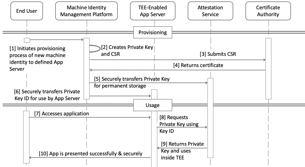
Figure 10 - Communication Flows between SKC, Trust Protection Platform, and CA
