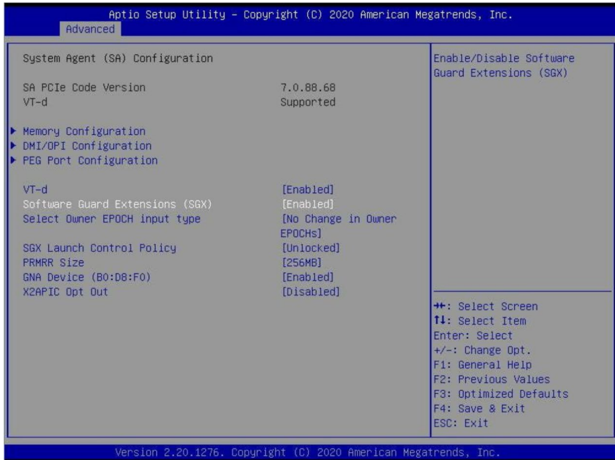
Figure 6 - BIOS Enable SGX
