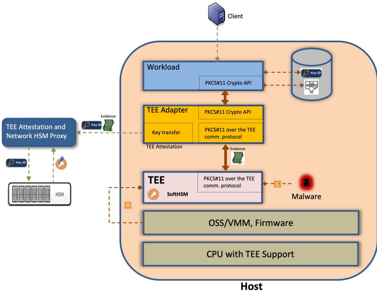
Figure 2 - Private Key Protection Flows
