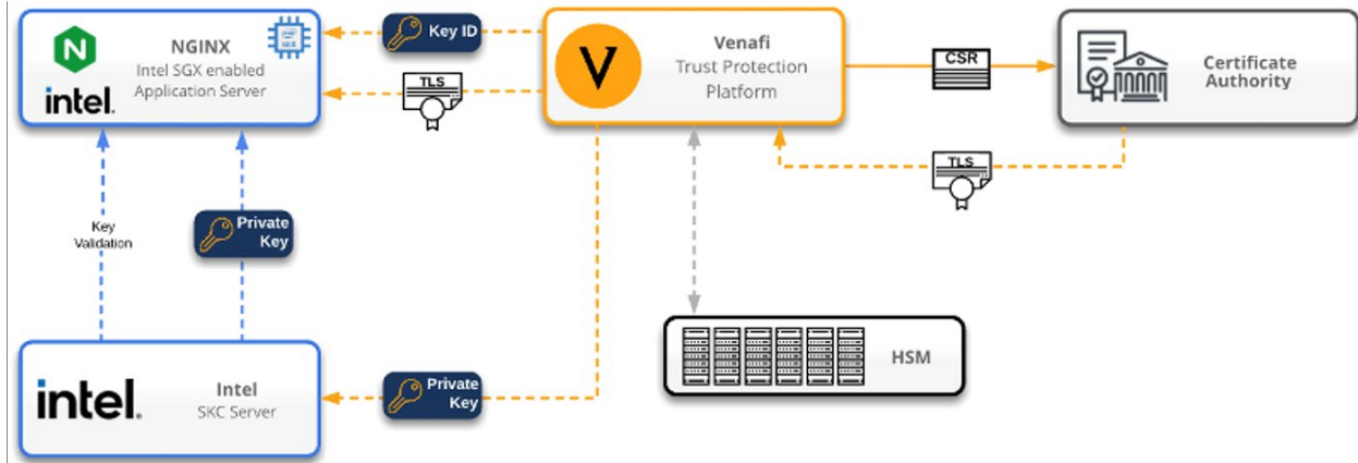
Figure 8 - End-to-End Machine Identity Lifecycle Management Platform
